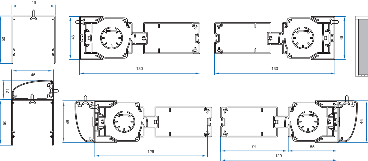
Profiles Sections
